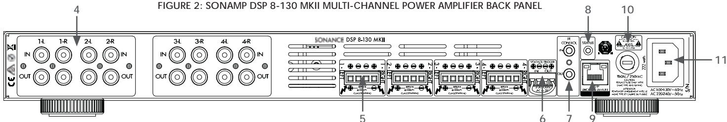
FIGURE 2: SONAMP DSP 8-130 MKII MULTI-CHANNEL POWER AMPLIFIER BACK PANEL
